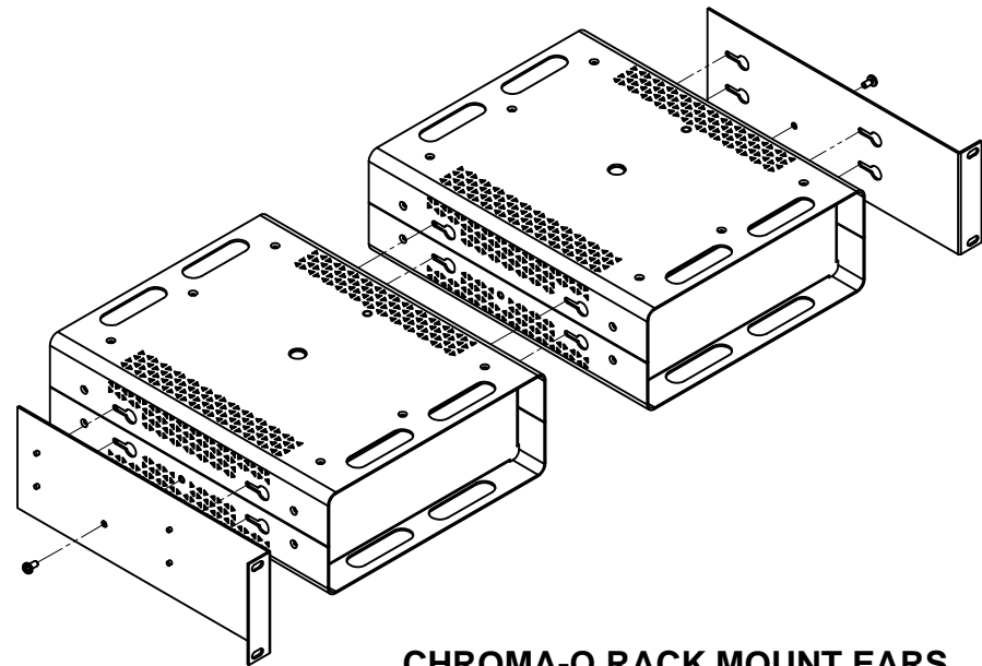
CHROMA-Q RACK MOUNT EARS DUAL UNIT (CHMBEAR)
